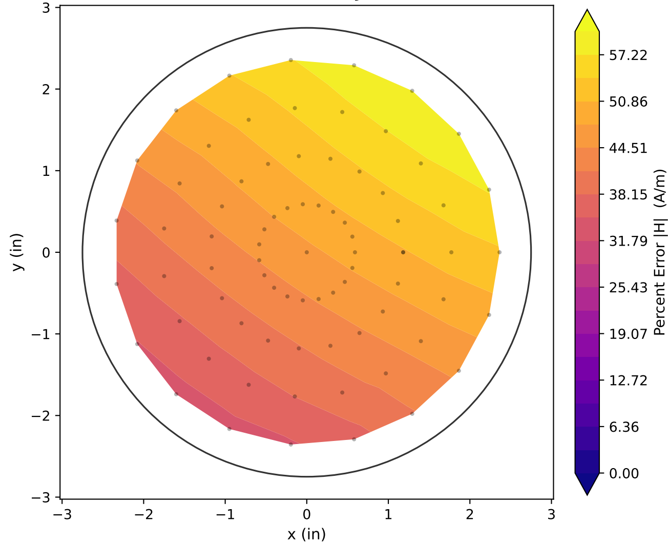
Reconstruction Error Percent — J=66.039 \text{ A/in}^2 , slice 3
